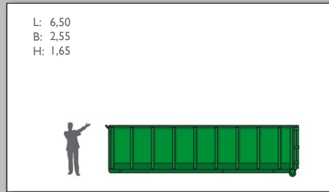
Abrollcontainer 22 m 3
