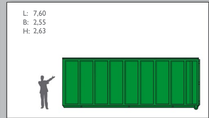
Abrollcontainer 40 m 3
